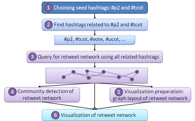
Figure 5. End-to-end analysis workflow in [9].
