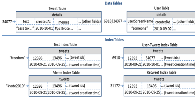
Figure 4. HBase tables for Truthy.
