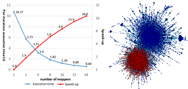
Figure 8. Per-iteration execution time for MRFR.
