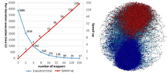
Figure 10. Per-iteration execution time of MRFR (2012).
