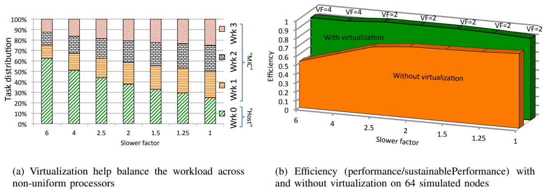
Fig. 6. The role of virtualization in enabling homogeneous programming in a heterogeneous computing environment
