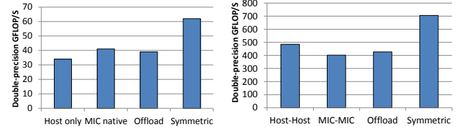
(a) Performance on 1 node. Grid size = 256x512x512 (b) Performance on 16 nodes. Grid size = 1024x1024x1024
