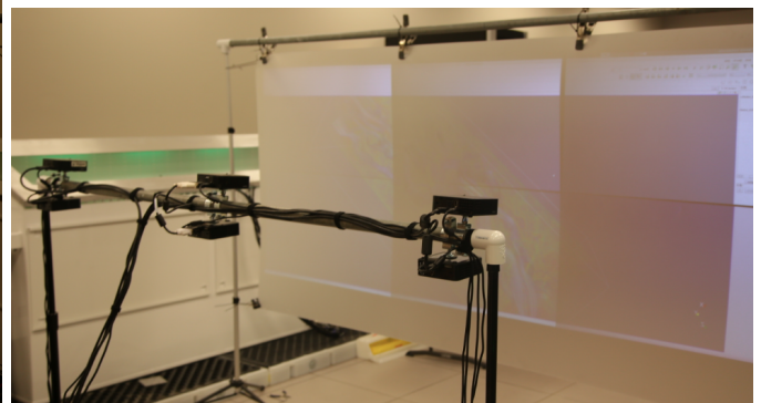
Fig. 4. Top Rear-projection setup with the Da-Lite Ultra Wide Angle screen, under fluorescent lighting at the SC2013 floor. By designing an enclosure from 80/20 aluminum framing, the picowall can achieve reasonable contrast in these environments despite low lumens. Bottom left : experimentation with inexpensive Lexan LED signage material. While hotspots were an issue, similar materials could ultimately provide an extremely low-cost screen with sufficient rigidity to enable touch. Bottom right : back view of the rear-projected picowall.
