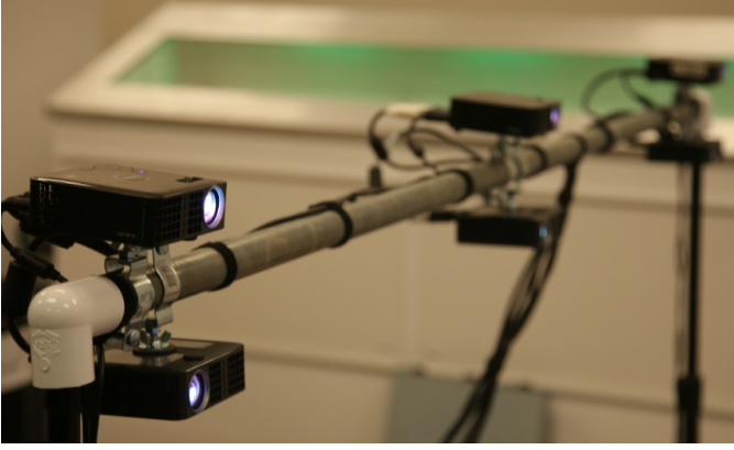
Fig. 2. Projector mount. We secure six projectors horizontally onto a single 6'×1.5" steel pipe, and use stainless steel brackets for individual mounts. Using microphone stands, the resulting construction is stiff. A similar outcome could be achieved with a sufficiently rigid photography backdrop kit.
