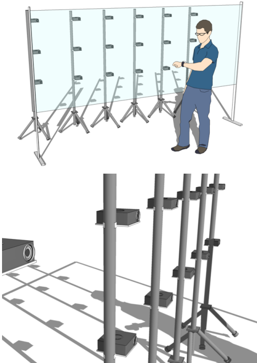
Fig. 1. Concept picowall module consisting of 18 projectors, driven by a single workstation with 6 outputs and six 3-way splitters. Projectors are mounted with lightweight, inexpensive photography equipment, designed for easy micro-adjustment.
