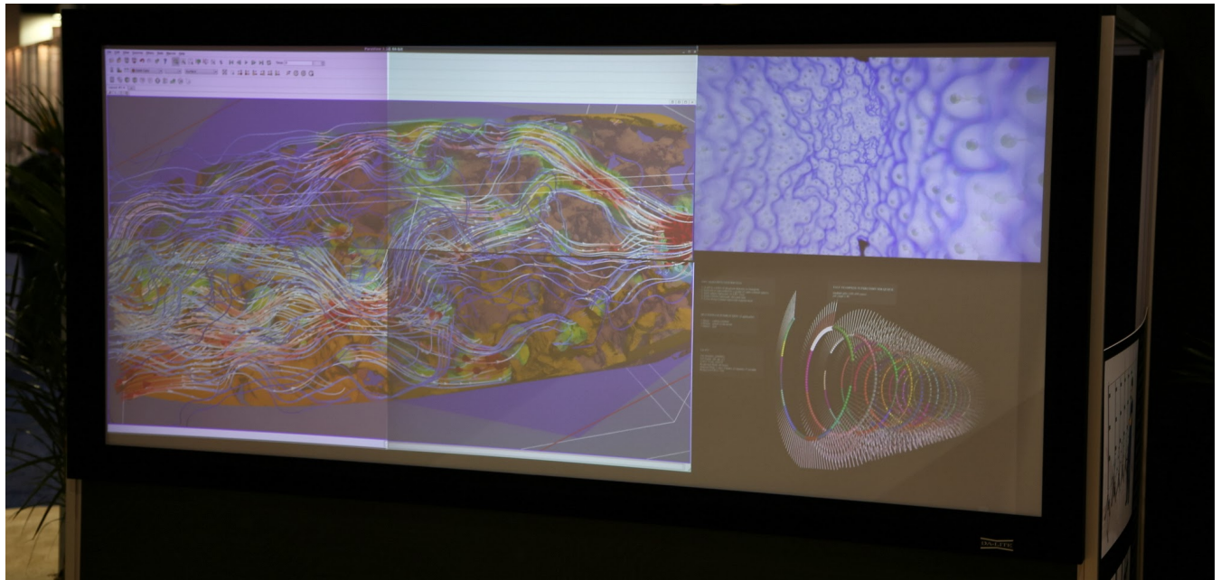
Fig. 3. Front-projected picowall prototype consisting of six 1280x800 Dell M110 projectors for a combined 3840x1600 resolution, driven by a single workstation with an ATI Radeon 5870 Eyefinity 6 GPU. Total weight of the projectors and mount is under 20 lbs.
