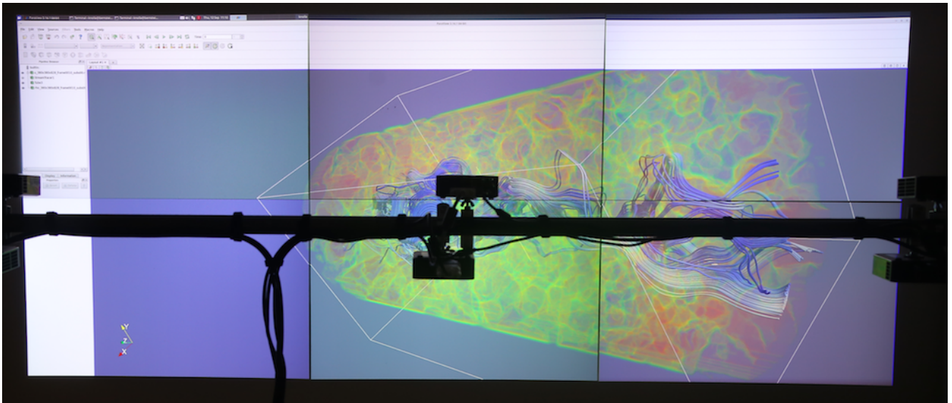
Fig. 3. Front-projected picowall prototype consisting of six 1280x800 Dell M110 projectors for a combined 3840x1600 resolution, driven by a single workstation with an ATI Radeon 5870 Eyefinity 6 GPU. Total weight of the projectors and mount is under 20 lbs.
